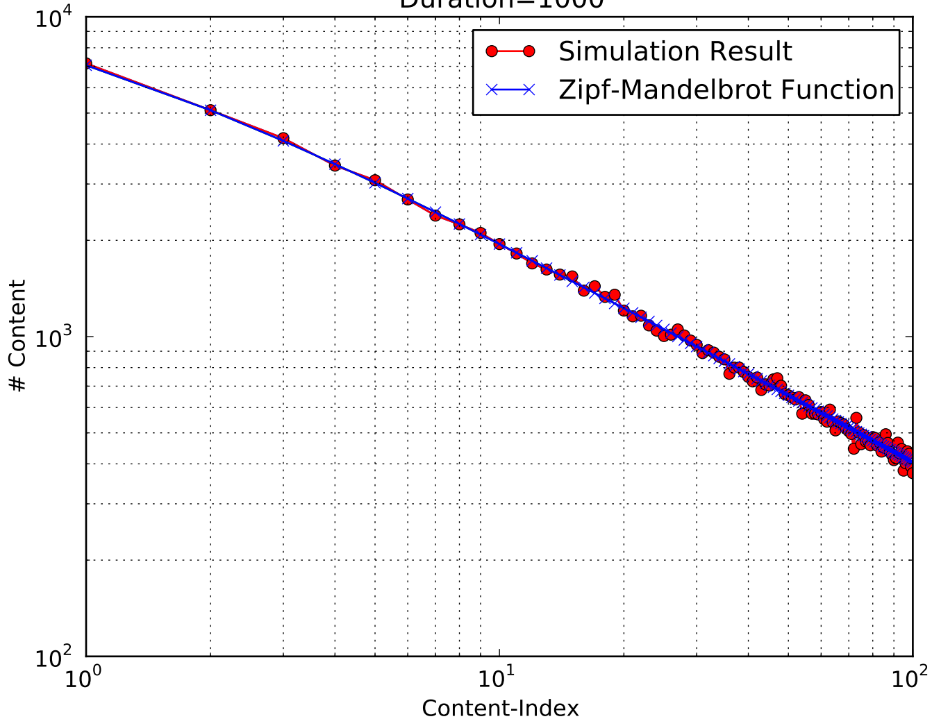
Comparsion Between Simulation and Theory Duration=1000
